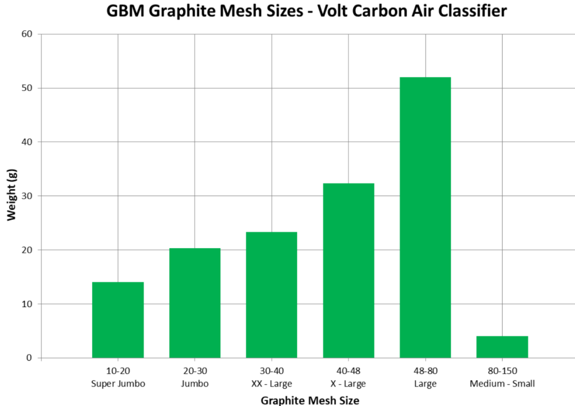
Figure 1: Flake size distribution from Air Classification: recovery of 146 g/kg of feedstock
